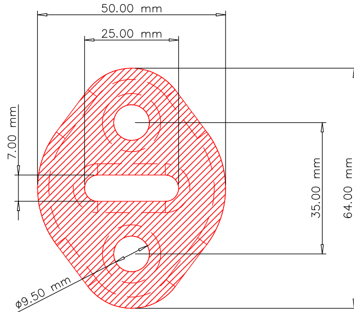
TOP VIEW (1 : 1)
